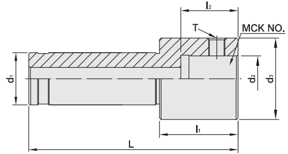
直柄 MCK 搪孔夾頭柄
